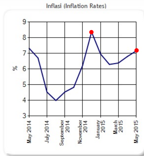
Time Series
